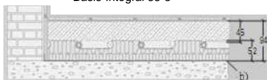
3. Installation mod opvarmede rum Basis-Integral 33-3
